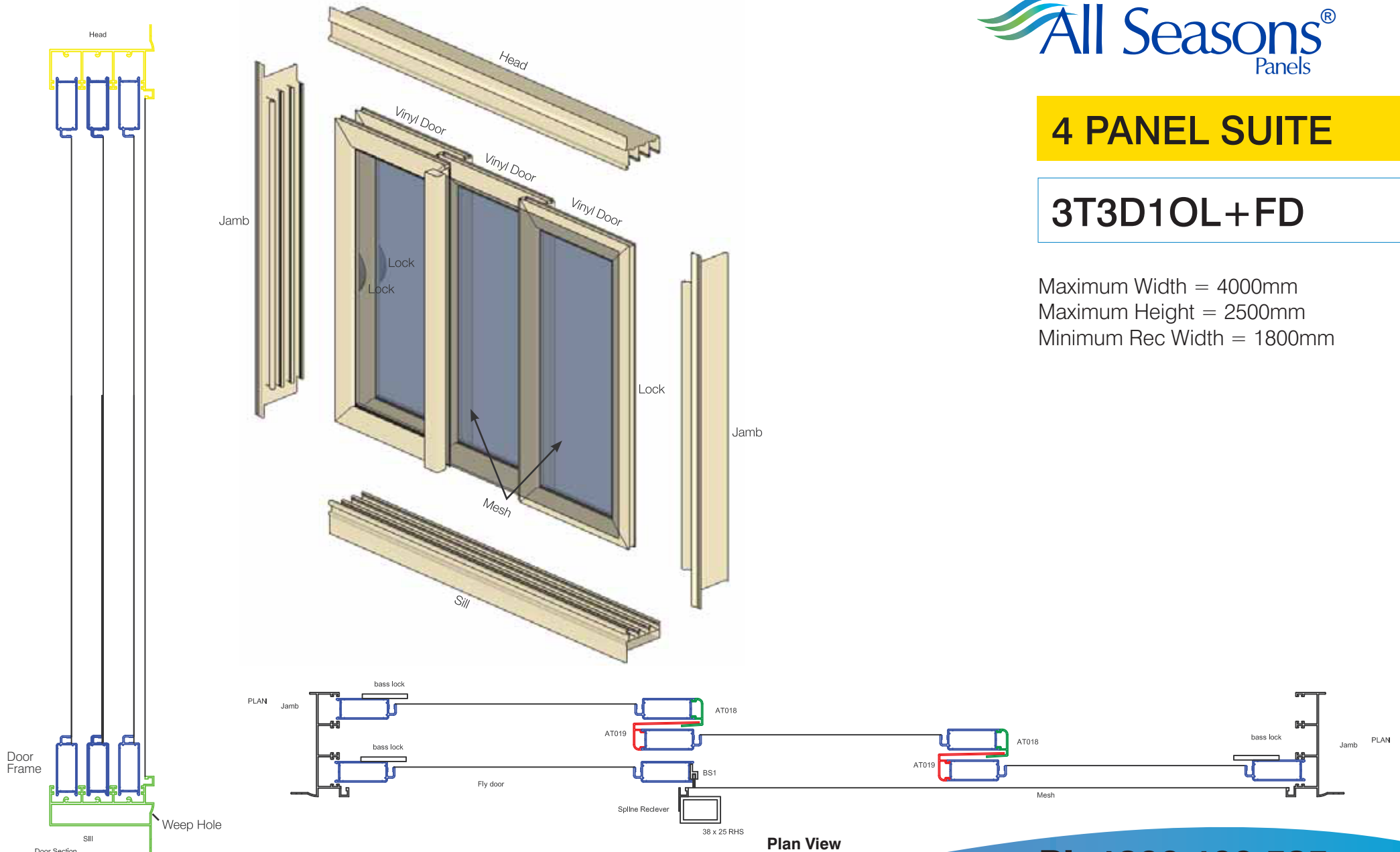
Section View
