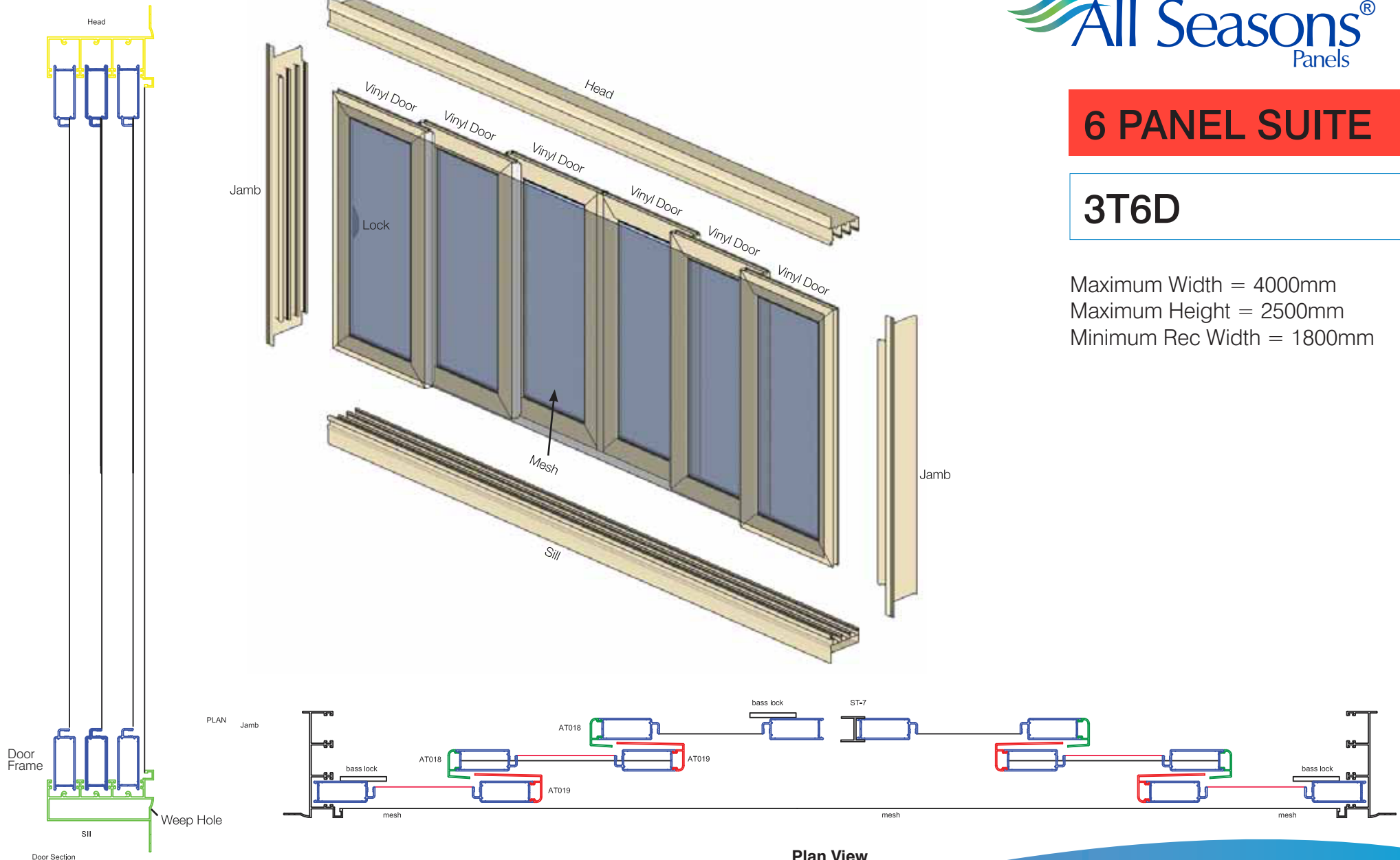
Plan View
